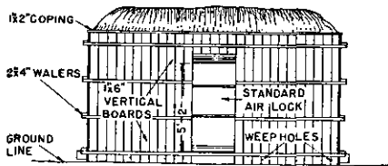
FRONT ELEVATION
