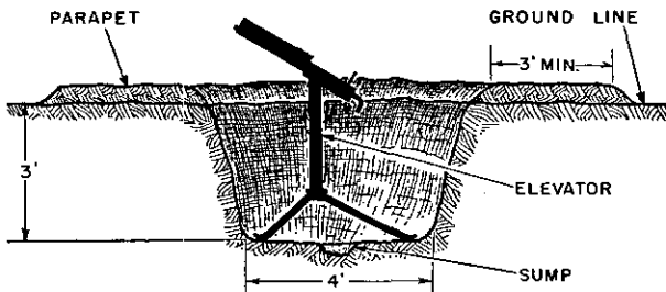
PROFILE
