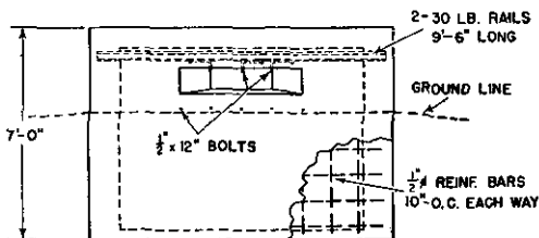
ELEVATION OF WALLS C & D
