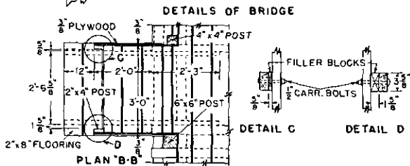
③ Framing plan of director platform and details of bridge.
